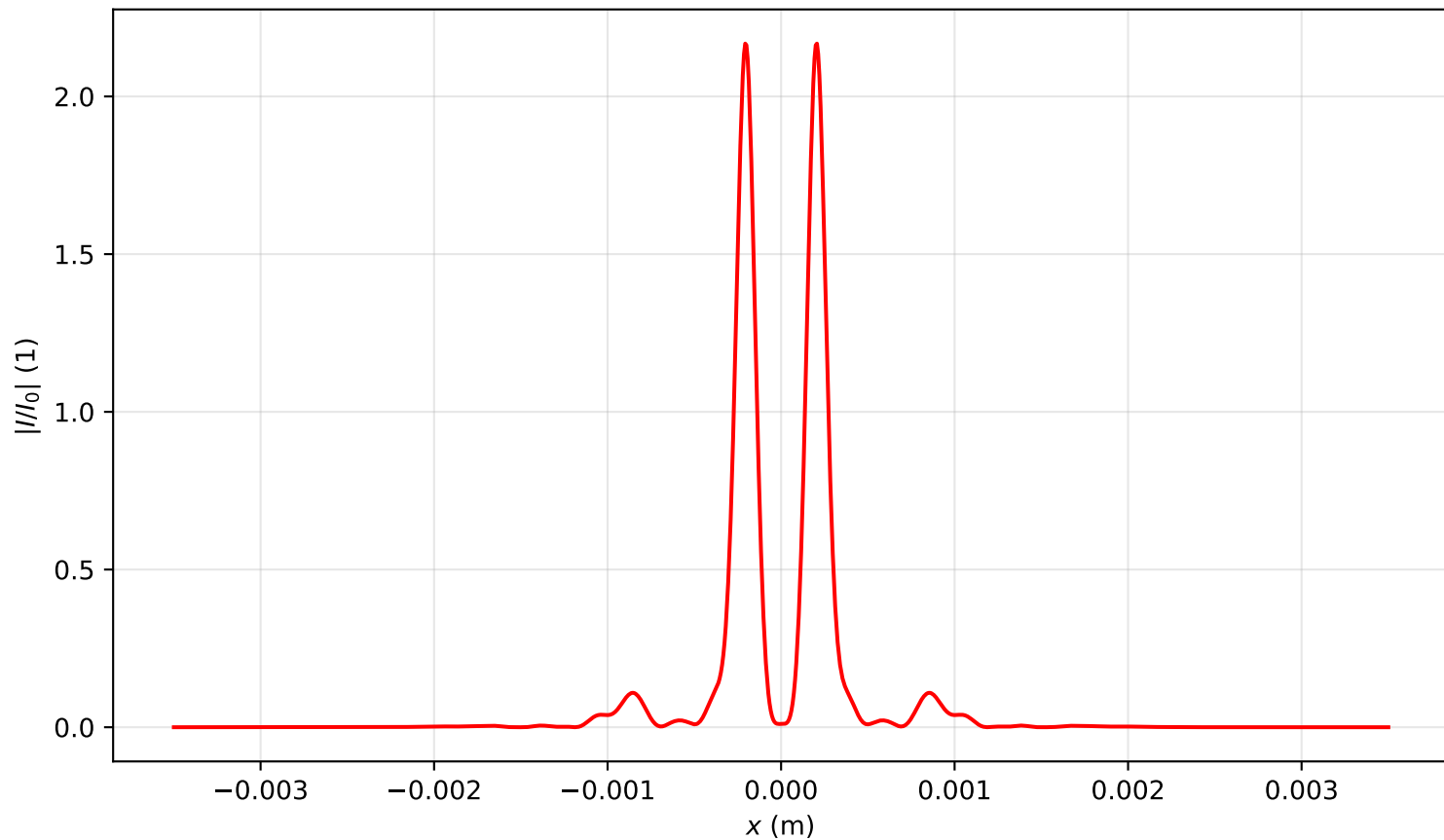
Intensity profile I(x, y = 0, z = 1.194)/I_0 , P_{in}=5.5P_{cr} , artificial time
